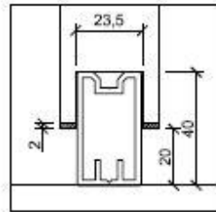
PILASTER FIXINGS floor
